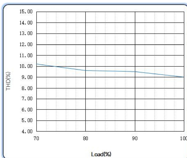
▲ Total Harmonic Distortion VS Load
